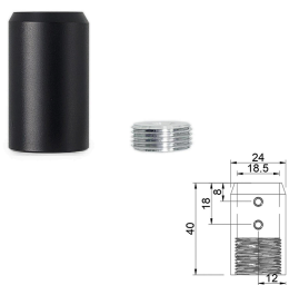
B款套座40 18管用 Type B Socket Base 40 - For 18 mm Tube
