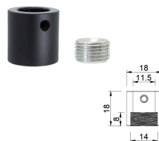
C款套座 11管用 Type C Socket Base - For 11 mm Tube
