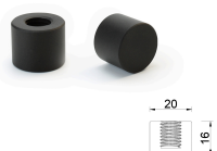
内牙层托堵头 15管用 Internally Threaded Shelf Support End Cap - For 15 mm Tube
