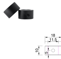
B款平托 11管用 Type B Flat Support - For 11 mm Tube
