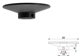
A款平托 11管用 Type A Flat Support - For 11 mm Tube
